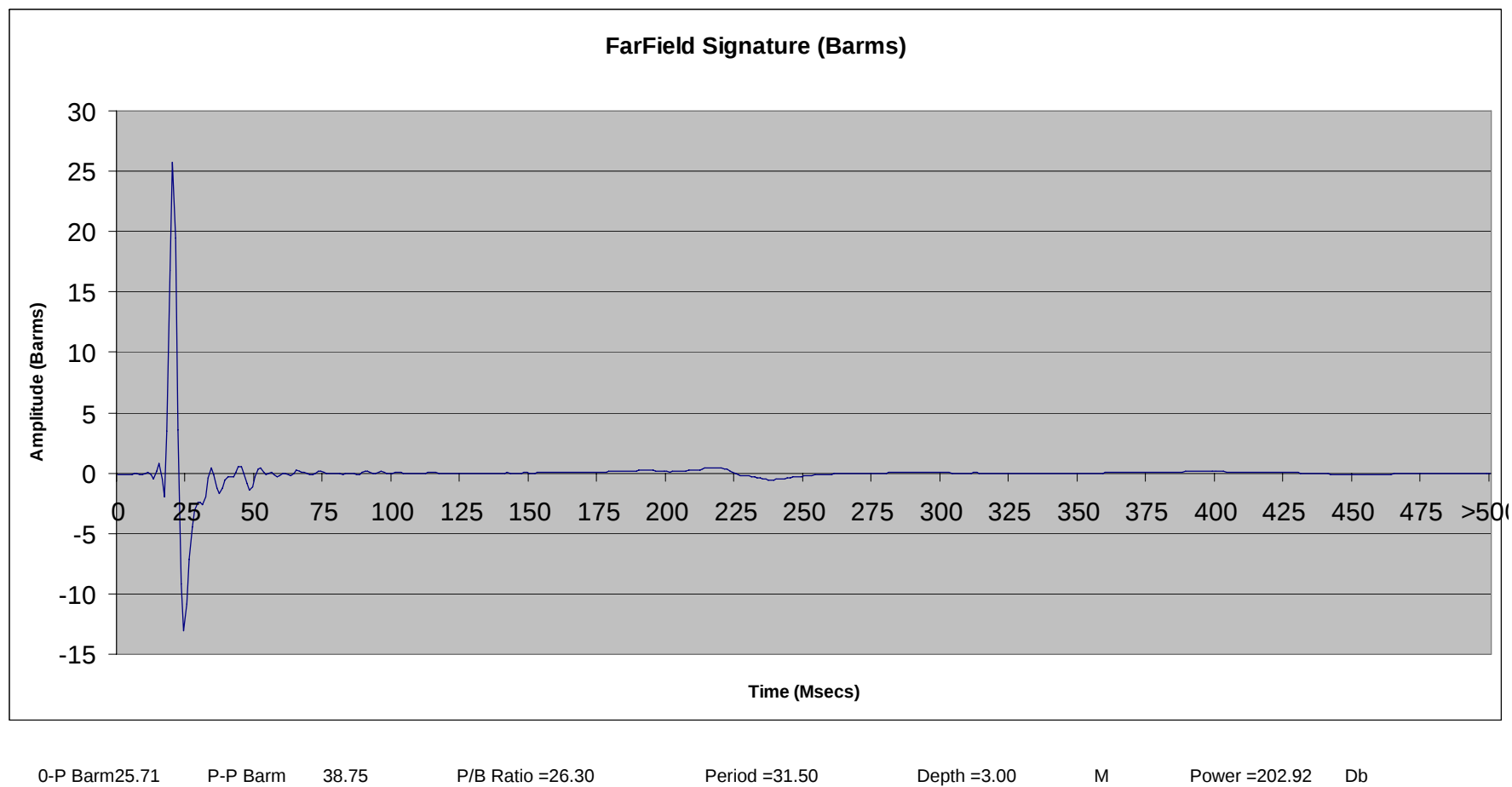
File 2.30: 2400 cu in Twin SeaScan Tri-Cluster ® array @ 10 ft
