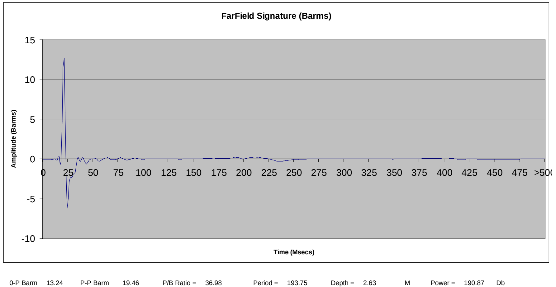
Figure 1: Time signature of the 1200 cu in Tri-Cluster ® array at a depth of 10 Feet (from fig 2.33)
