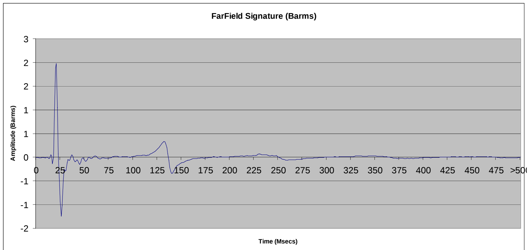
File 2.60: 150 cu in SeaScan Tri-Cluster ® array (# 3 only) @ 10 ft
