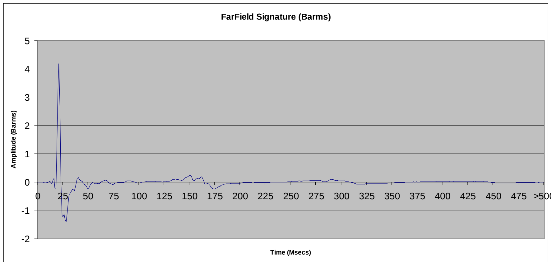
File 2.43: 600 cu in SeaScan Tri-Cluster ® array @ 10 ft
