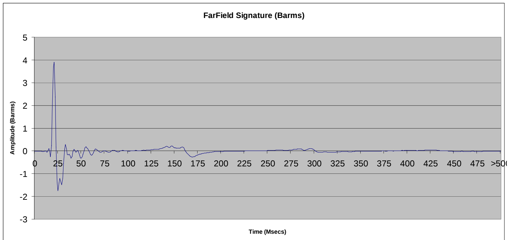
File 2.77: 300 cu in SeaScan Tri-Cluster ® array (#5 & 6) @ 10 ft
