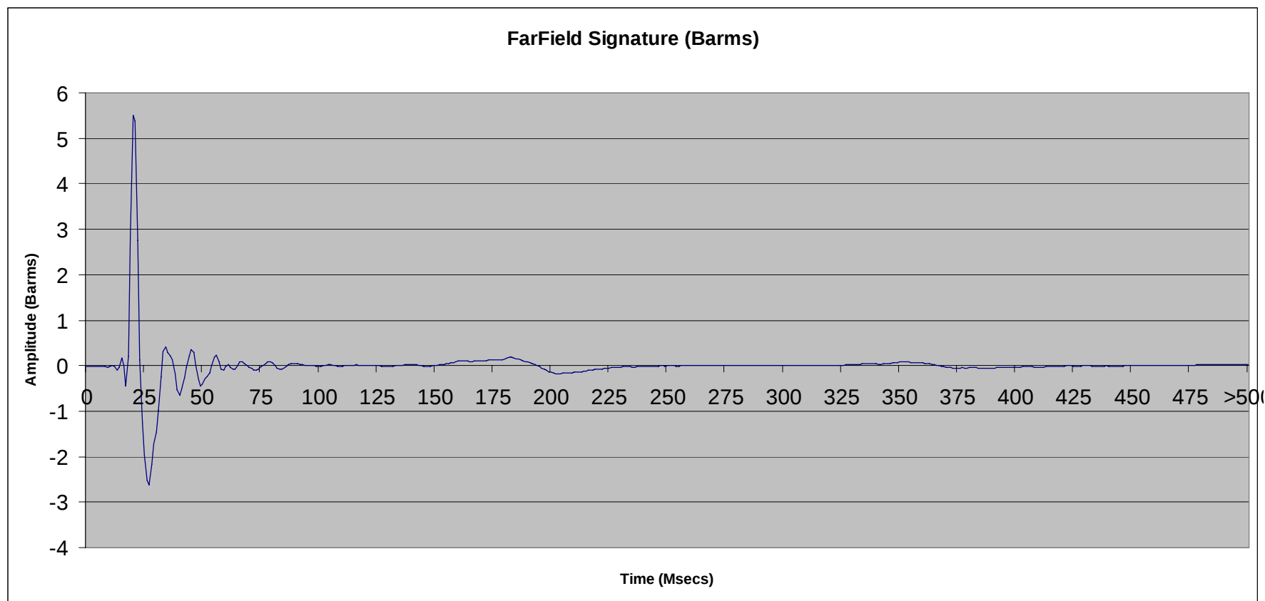
File 2.82: 600 cu in SeaScan Tri-Cluster ® array (#3,4,5,6 only) @ 10 ft
