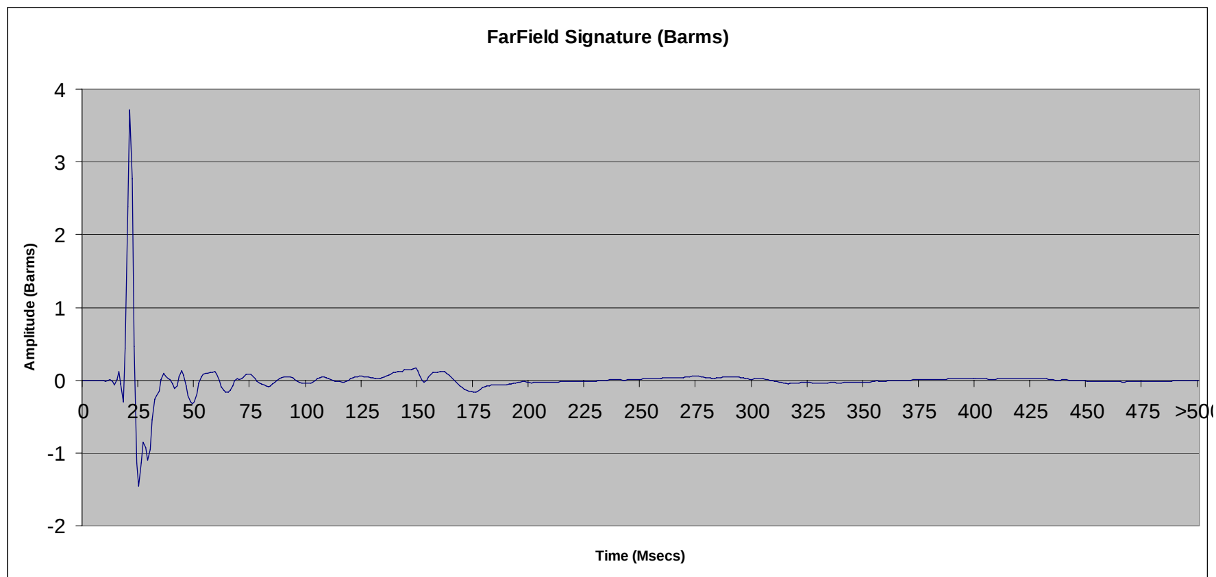
File 2.69: 150 cu in SeaScan Tri-Cluster ® array (#5 only) @ 10 ft
