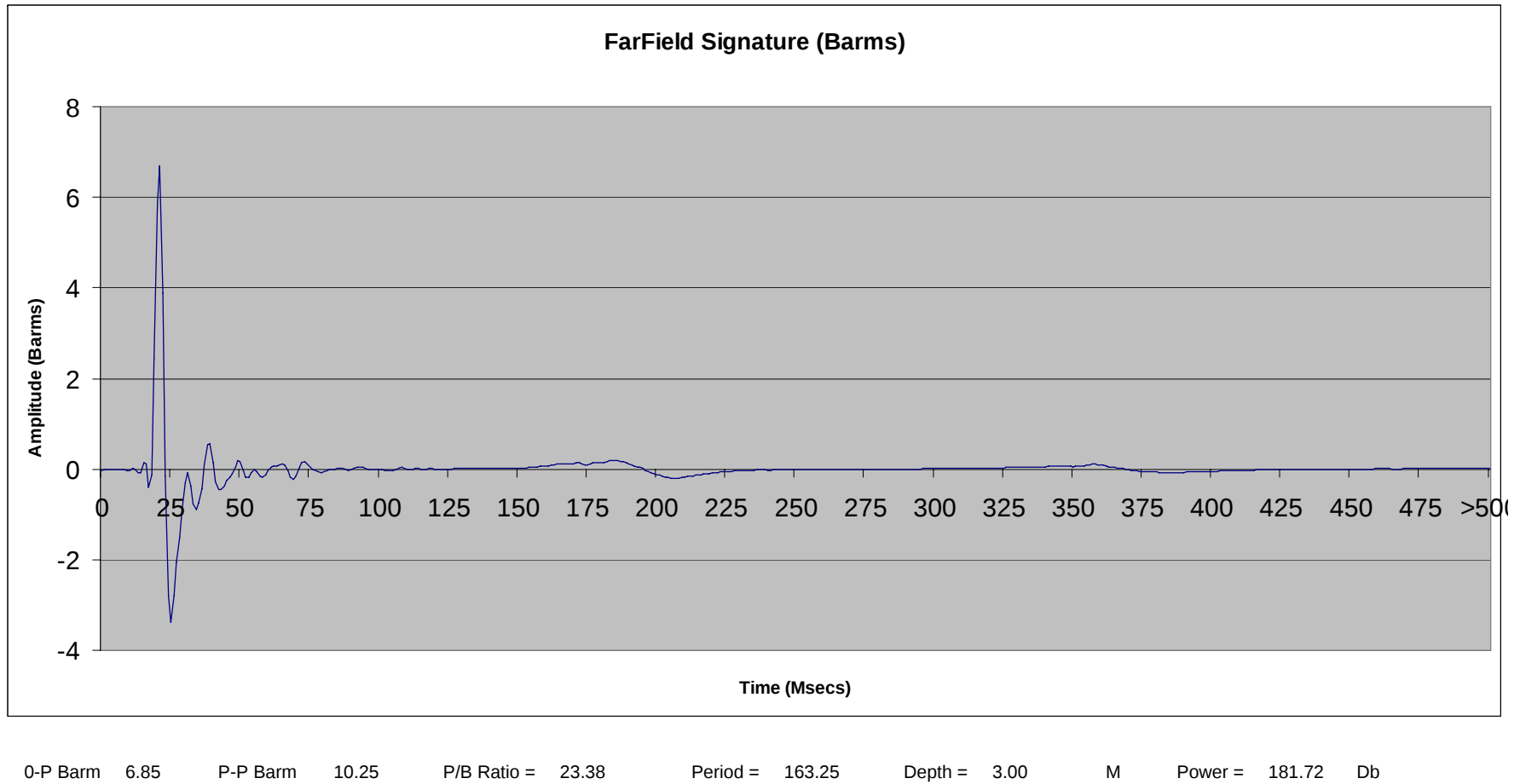
File 2.38: 600 cu in SeaScan Tri-Cluster ® array @ 10 ft
