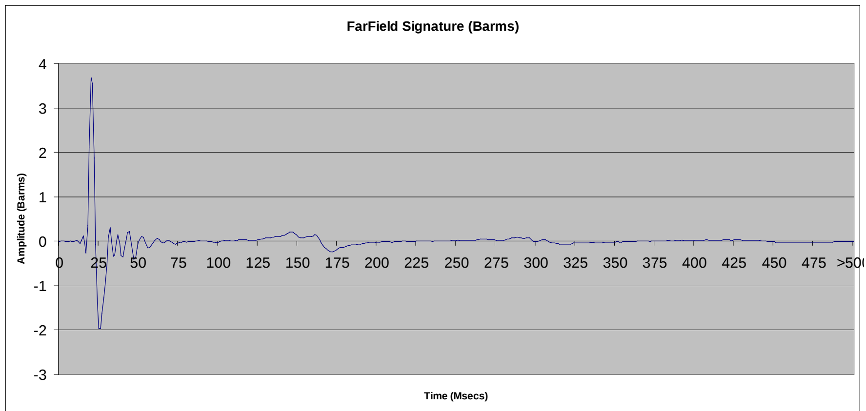
File 2.55: 150 cu in SeaScan Tri-Cluster ® array (# 8 only) @ 10 ft
