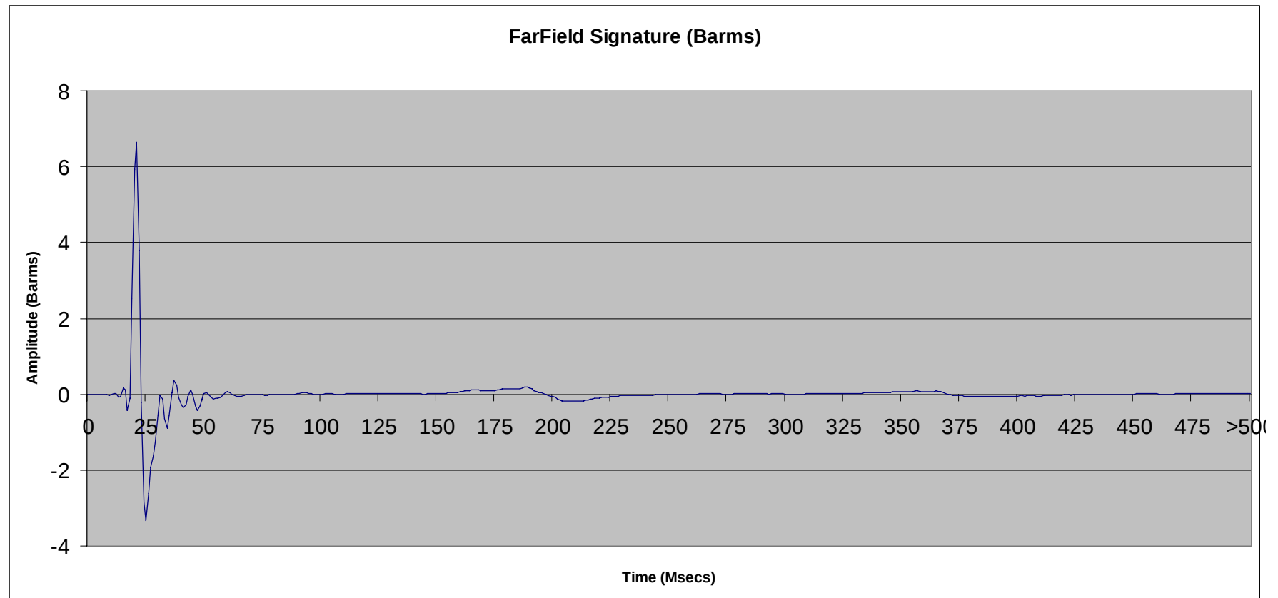
File 2.39: 600 cu in SeaScan Tri-Cluster ® array @ 10 ft
