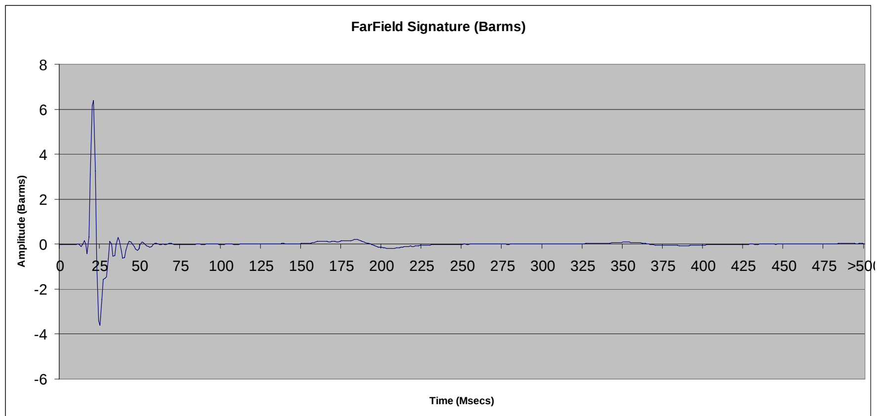
File 2.81: 600 cu in SeaScan Tri-Cluster ® array (#3,4,5,6 only) @ 10 ft
