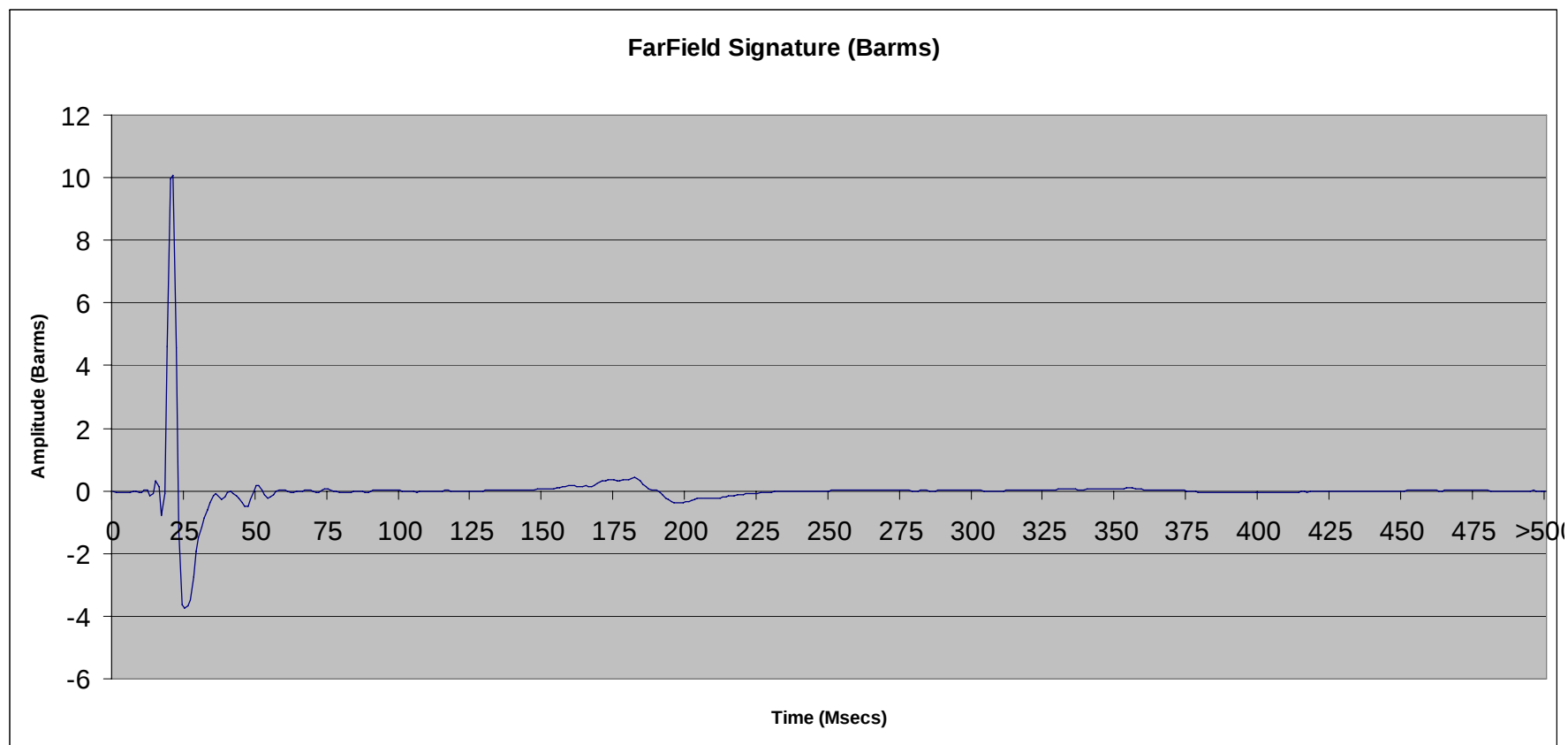
File 2.96: 900 cu in SeaScan Tri-Cluster ® array (#1,2,5,6,7,8 only) @ 10 ft
