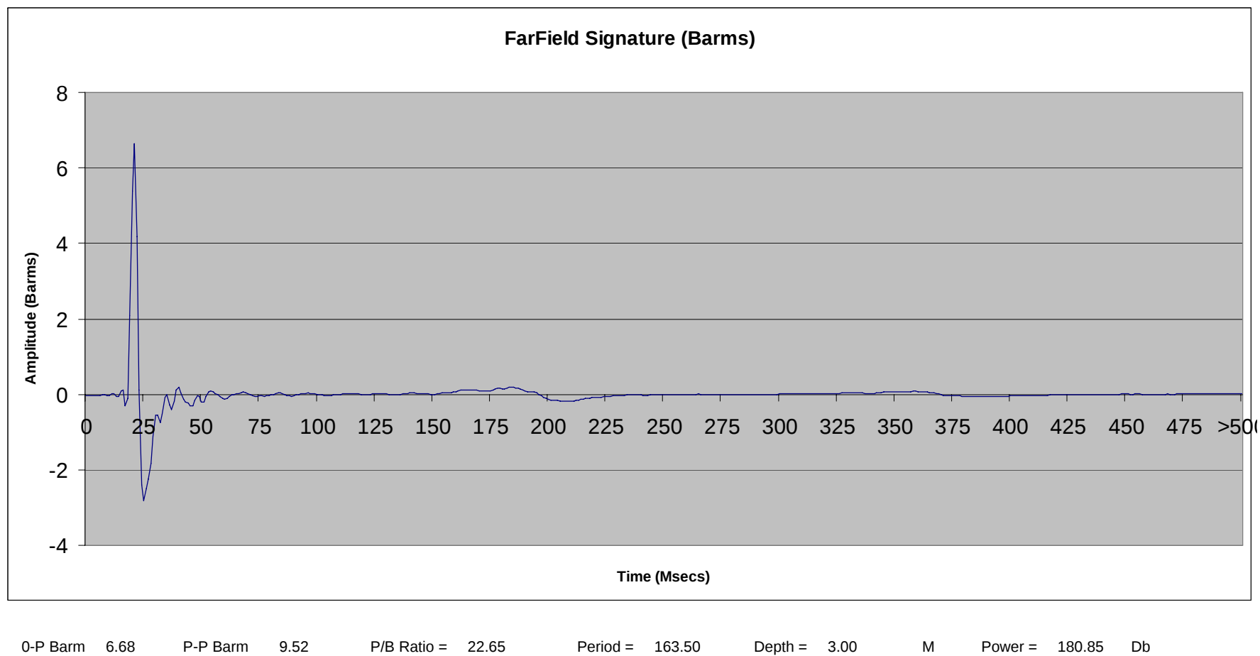
File 2.78: 600 cu in SeaScan Tri-Cluster ® array (#3,4,5,6 only) @ 10 ft
