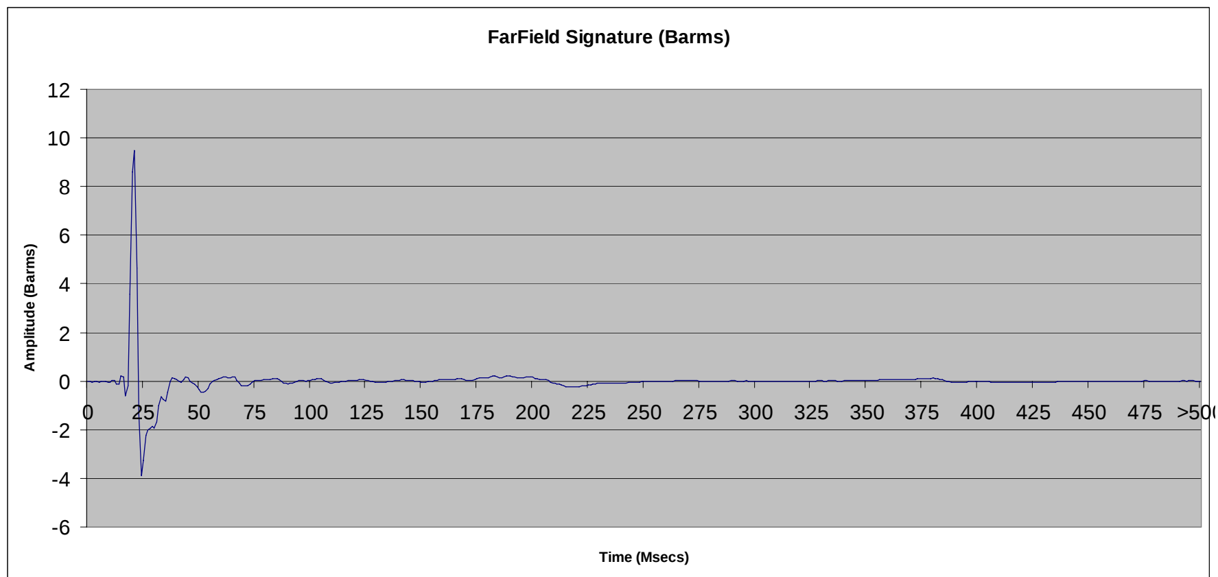
File 2.85: 900 cu in SeaScan Tri-Cluster ® array (#1,2,3,4,5,6 only) @ 10 ft
