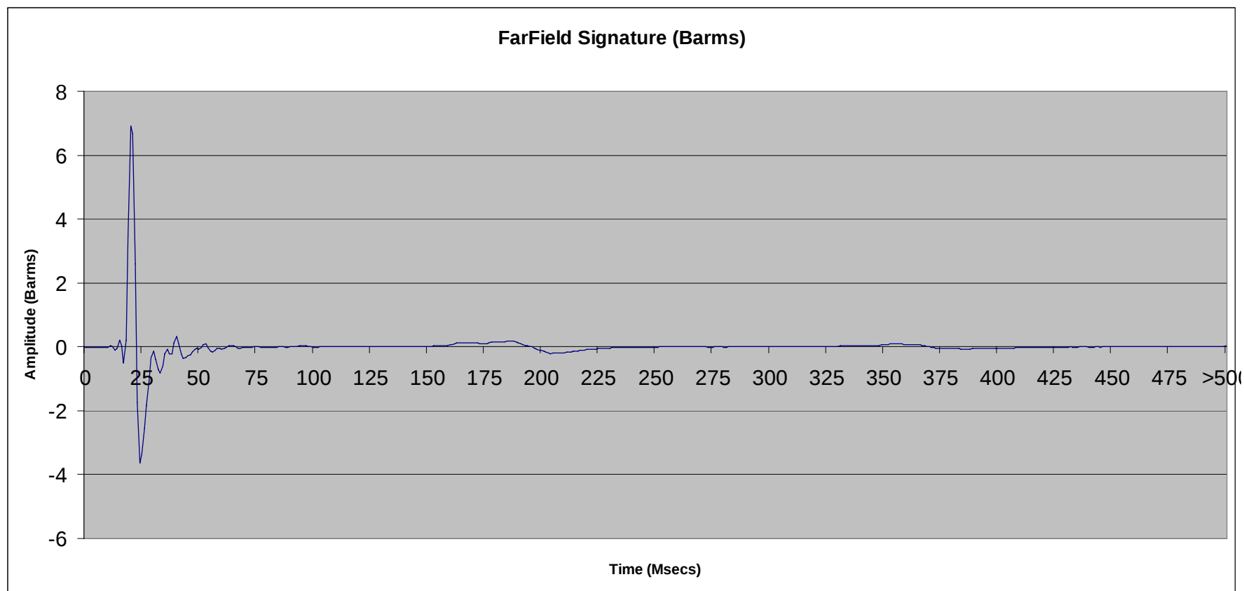
File 2.40: 600 cu in SeaScan Tri-Cluster ® array @ 10 ft
