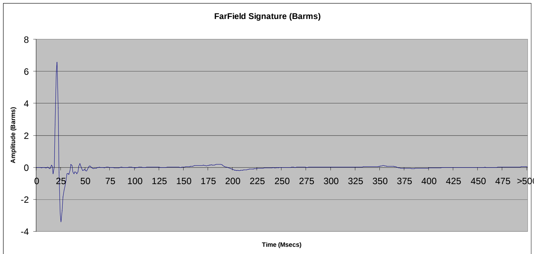
File 2.80: 600 cu in SeaScan Tri-Cluster ® array (#3,4,5,6 only) @ 10 ft
