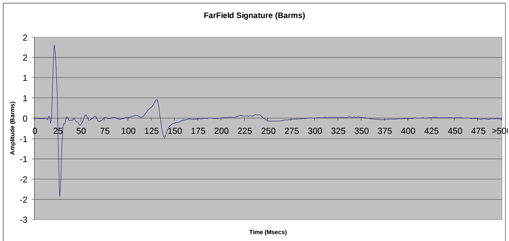
File 2.59: 150 cu in SeaScan Tri-Cluster ® array (# 8 only) @ 10 ft
