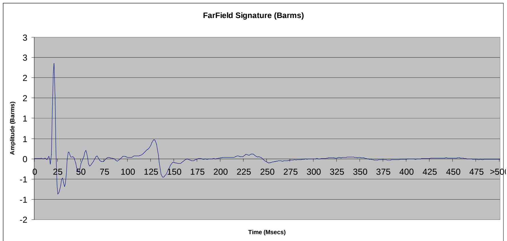
File 2.72: 150 cu in SeaScan Tri-Cluster ® array (#5 only) @ 10 ft
