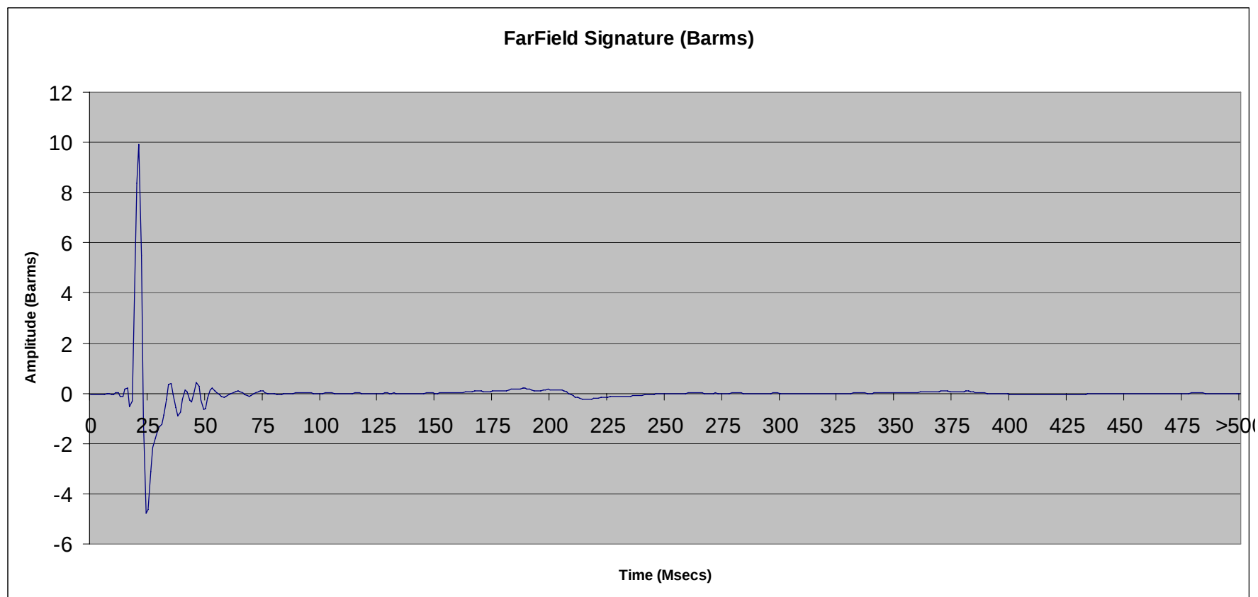
File 2.87: 900 cu in SeaScan Tri-Cluster ® array (#1,2,3,4,5,6 only) @ 10 ft
