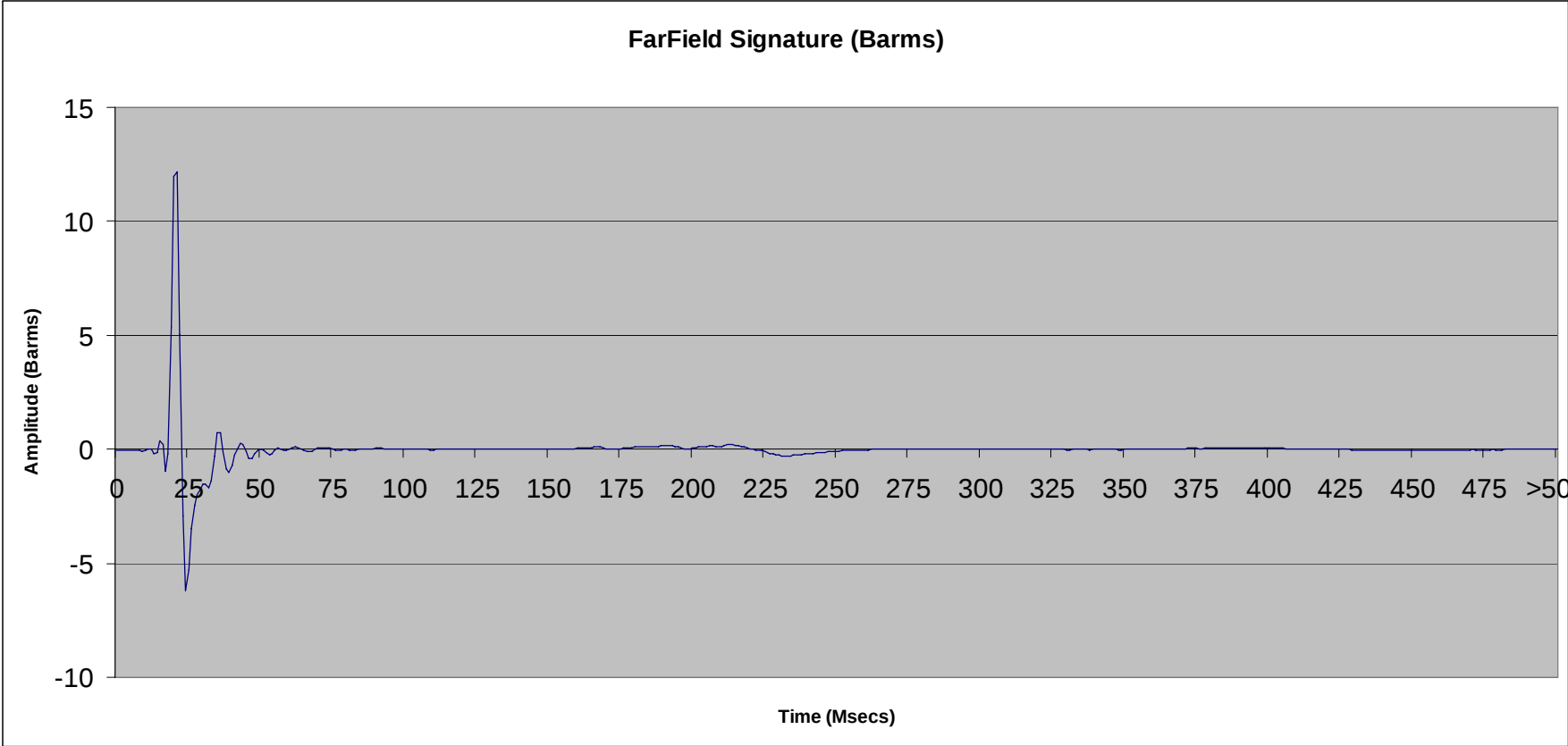
File 2.92: 1200 cu in Single Tri-Cluster ® Tri-Cluster array @ 10 ft
