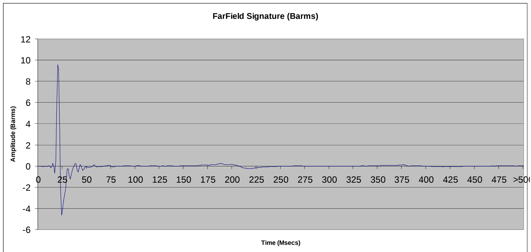
File 2.83: 900 cu in SeaScan Tri-Cluster ® array (#1,2,3,4,5,6 only) @ 10 ft
