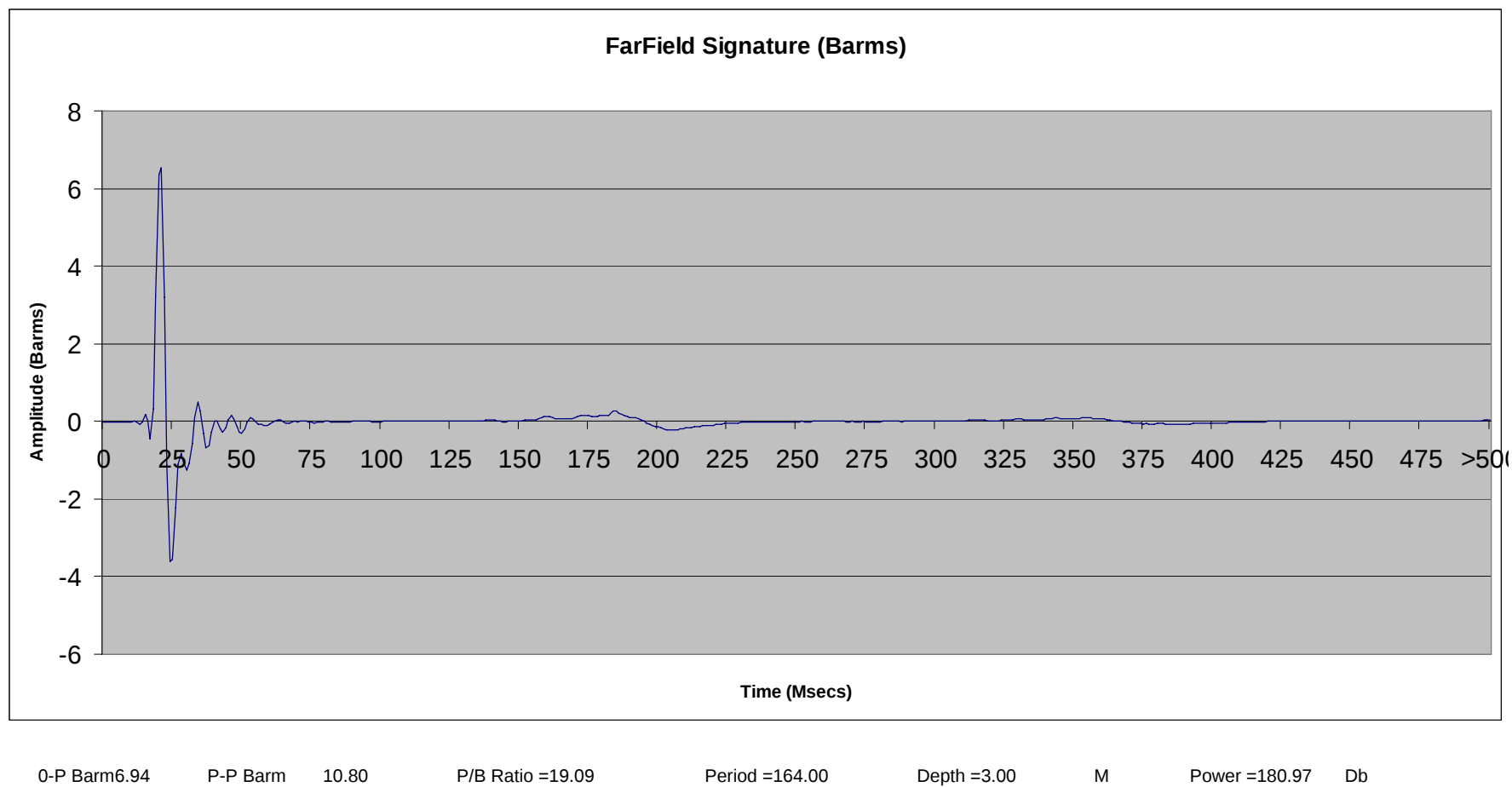
File 2.42: 600 cu in SeaScan Tri-Cluster ® array @ 10 ft
