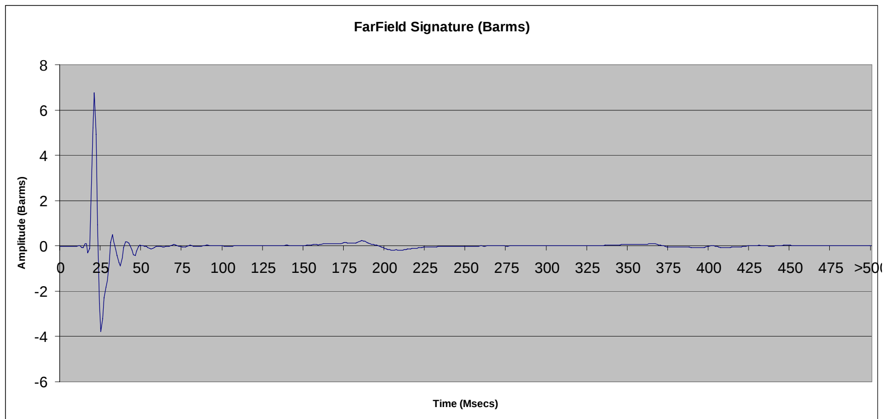
File 2.79: 600 cu in SeaScan Tri-Cluster ® array (#3,4,5,6 only) @ 10 ft
