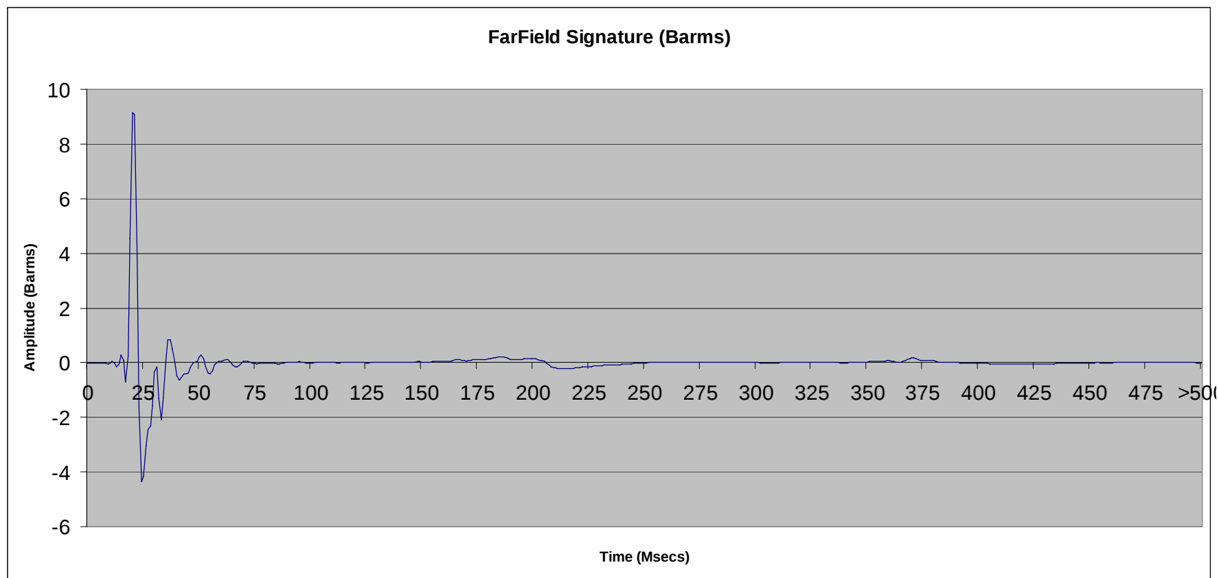
File 2.86: 900 cu in SeaScan Tri-Cluster ® array (#1,2,3,4,5,6 only) @ 10 ft
