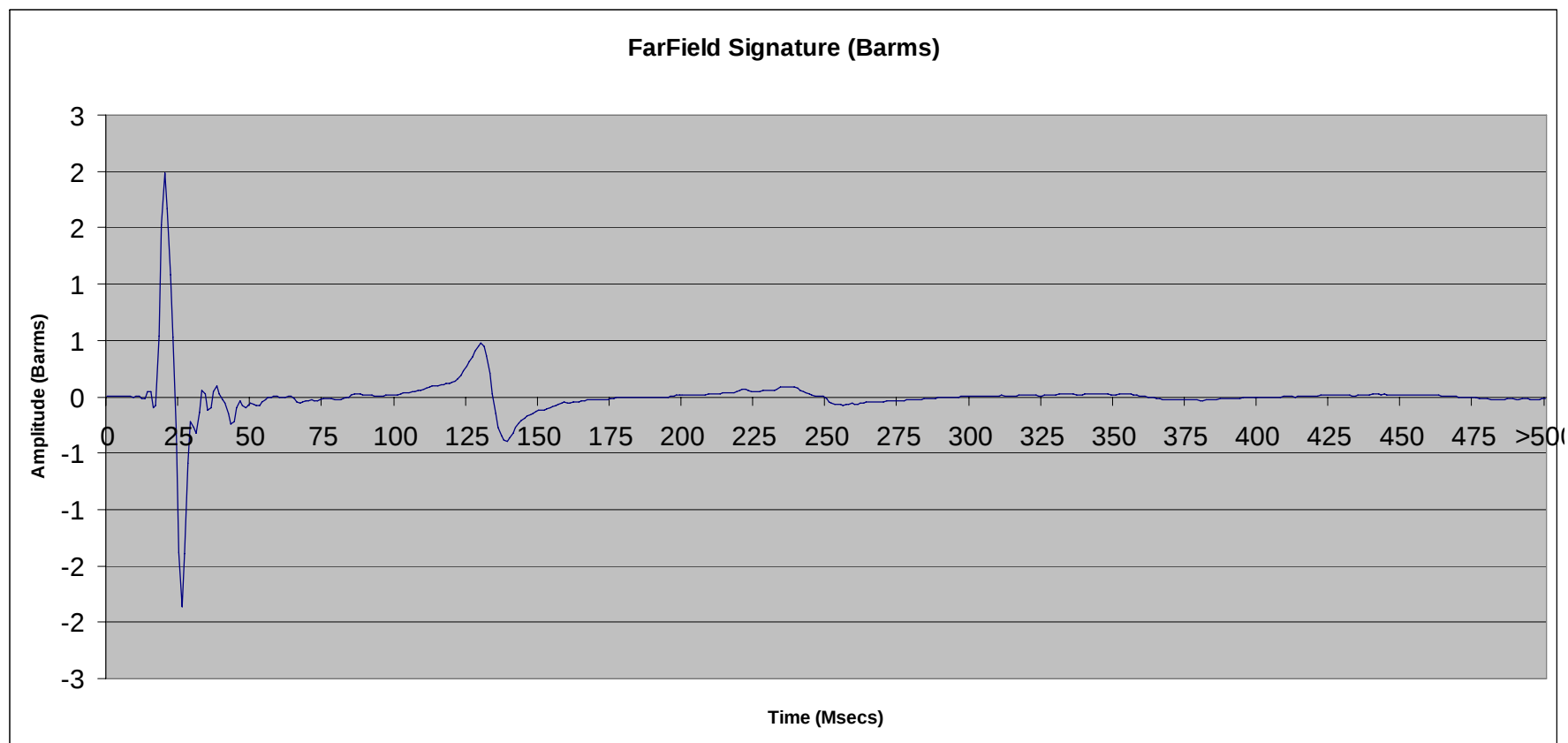
File 2.57: 150 cu in SeaScan Tri-Cluster ® array (# 8 only) @ 10 ft
