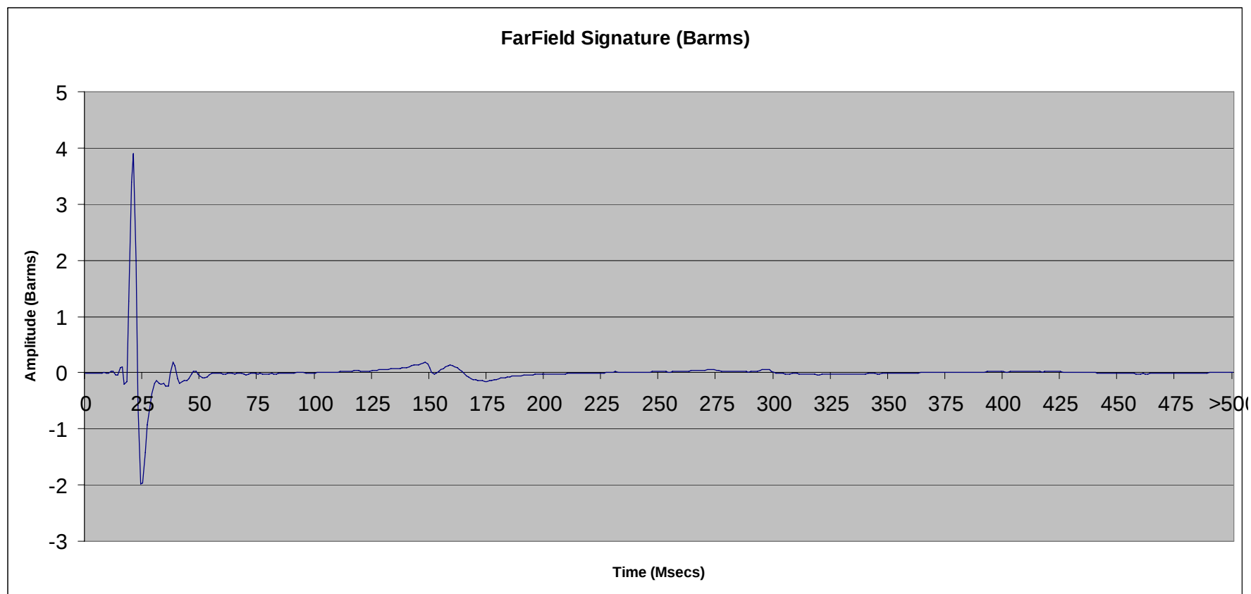
File 2.68: 300 cu in SeaScan Tri-Cluster ® array (# 3 & 4 only) @ 10 ft
