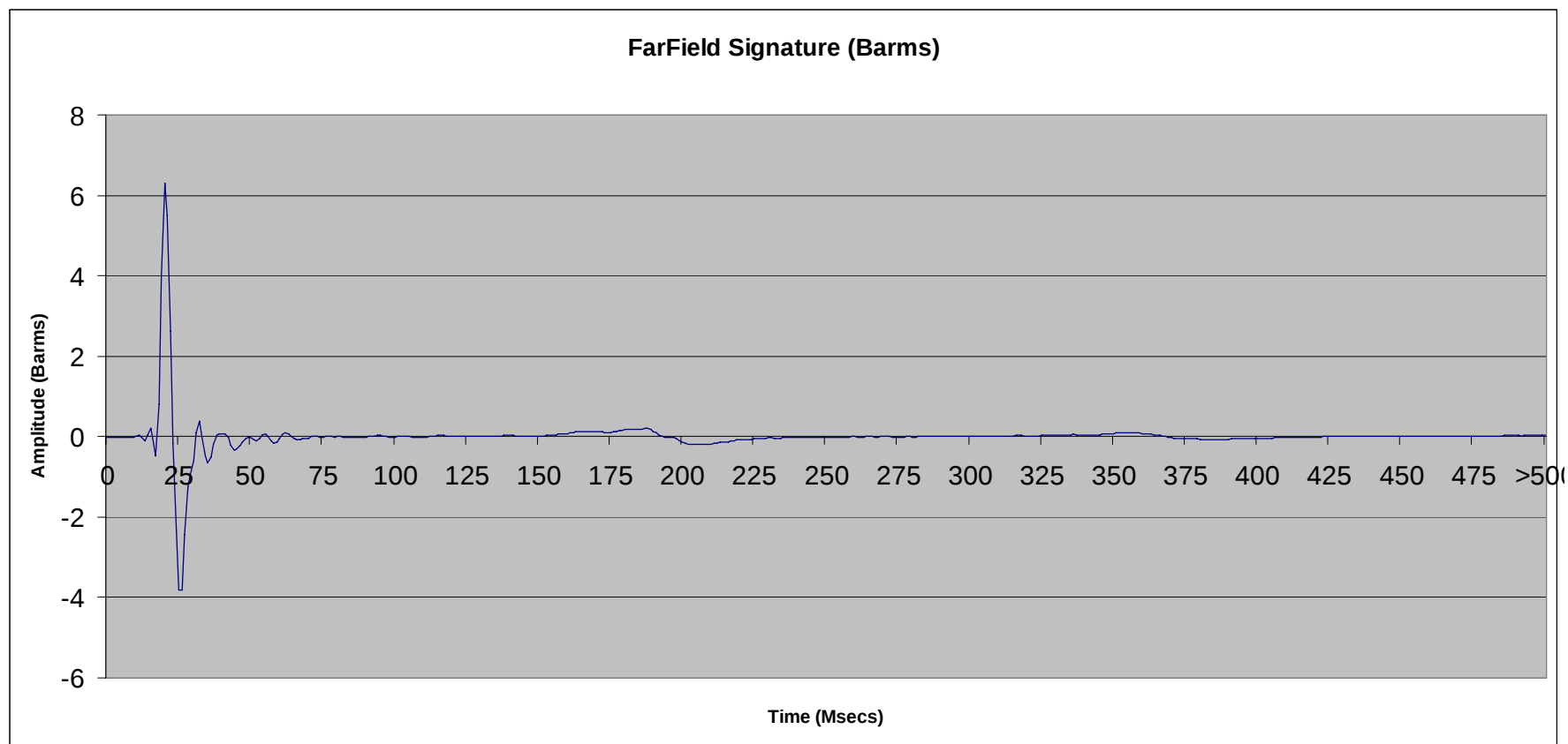
File 2.41: 600 cu in SeaScan Tri-Cluster ® array @ 10 ft
