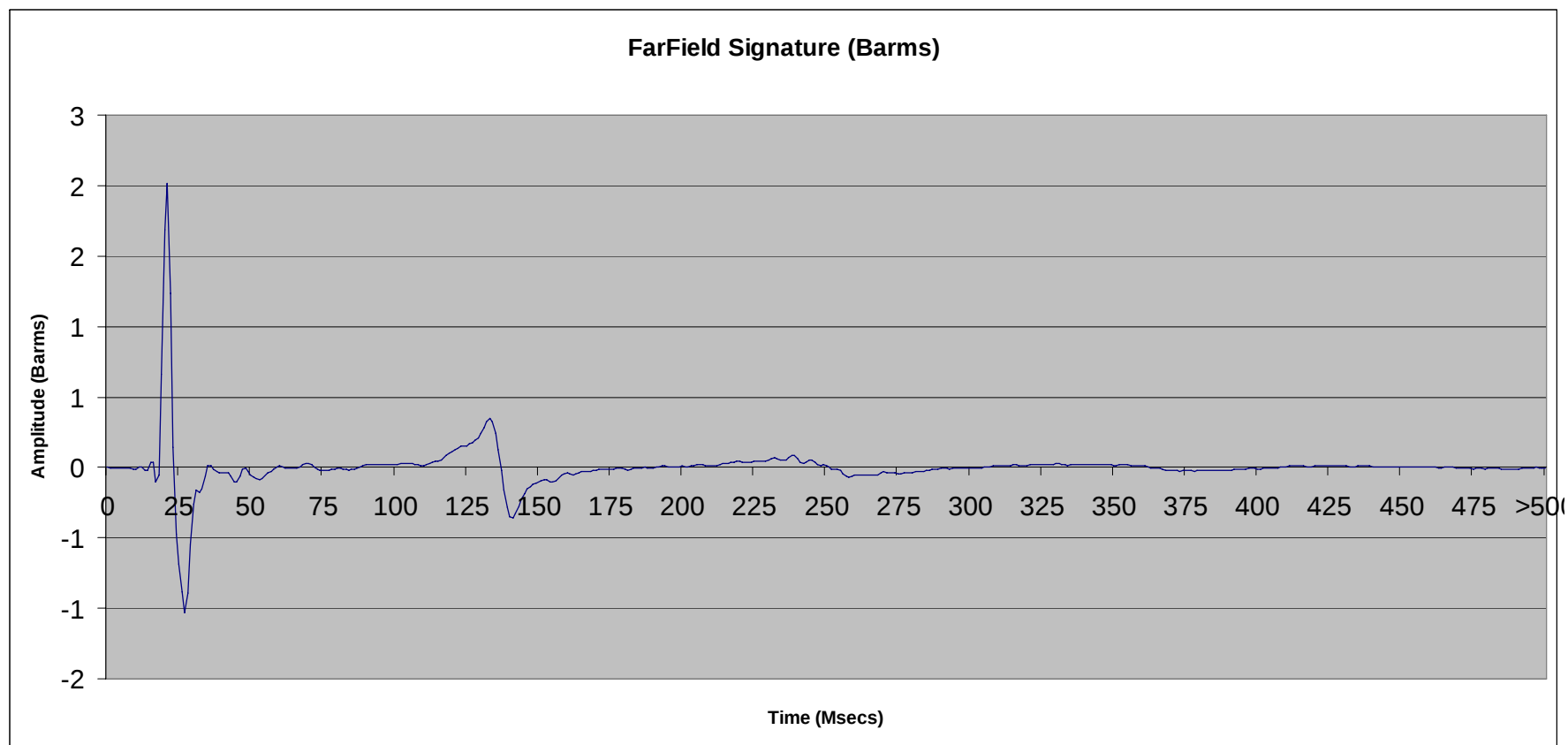
File 2.63: 150 cu in SeaScan Tri-Cluster ® array (# 3 only) @ 10 ft
