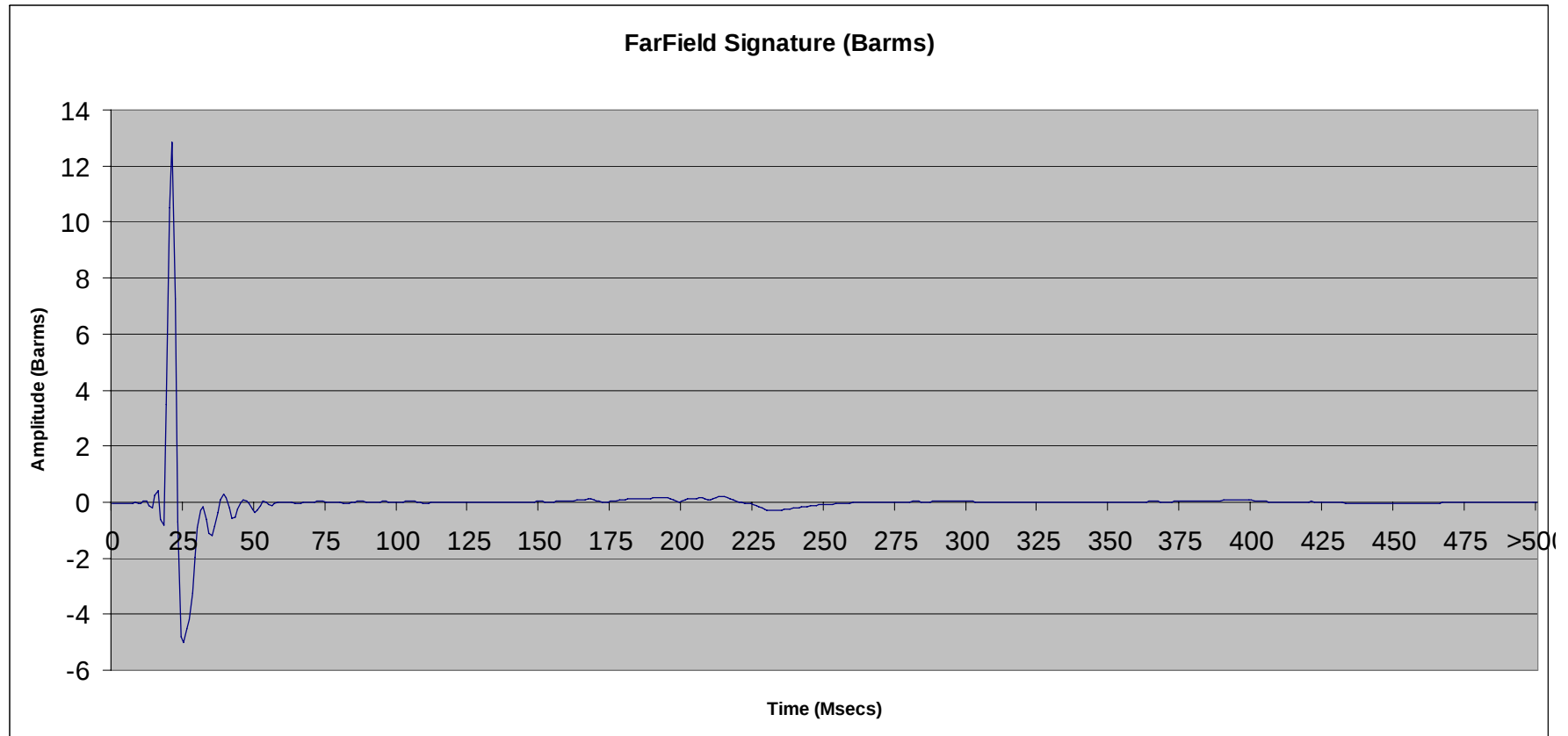
File 2.90: 1200 cu in Single Tri-Cluster ® Tri-Cluster array @ 10 ft
