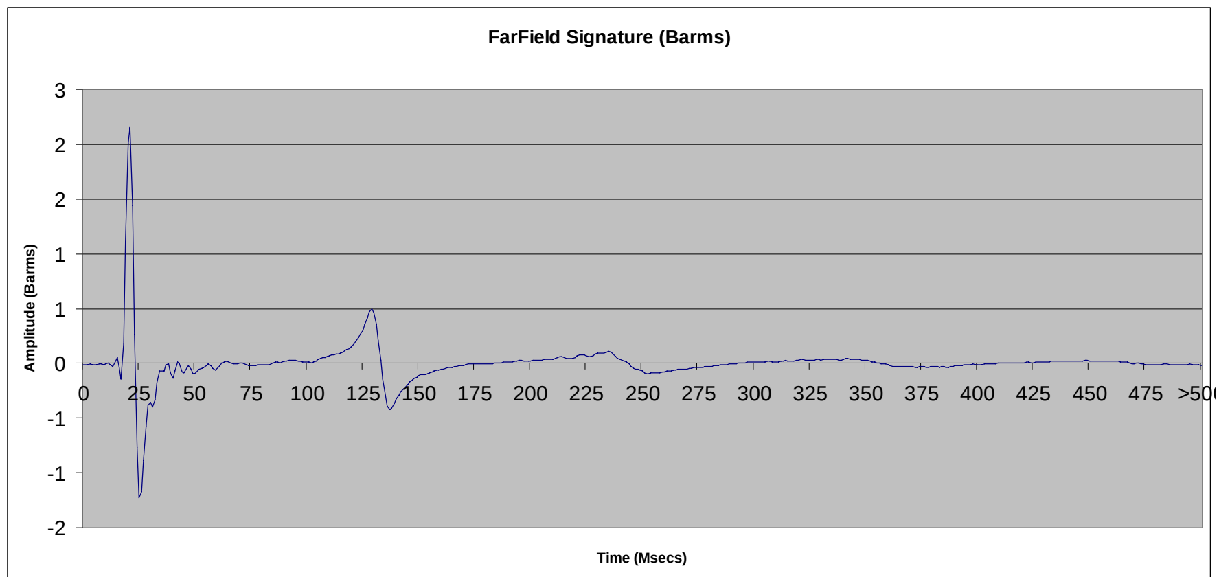
File 2.58: 150 cu in SeaScan Tri-Cluster ® array (# 8 only) @ 10 ft
