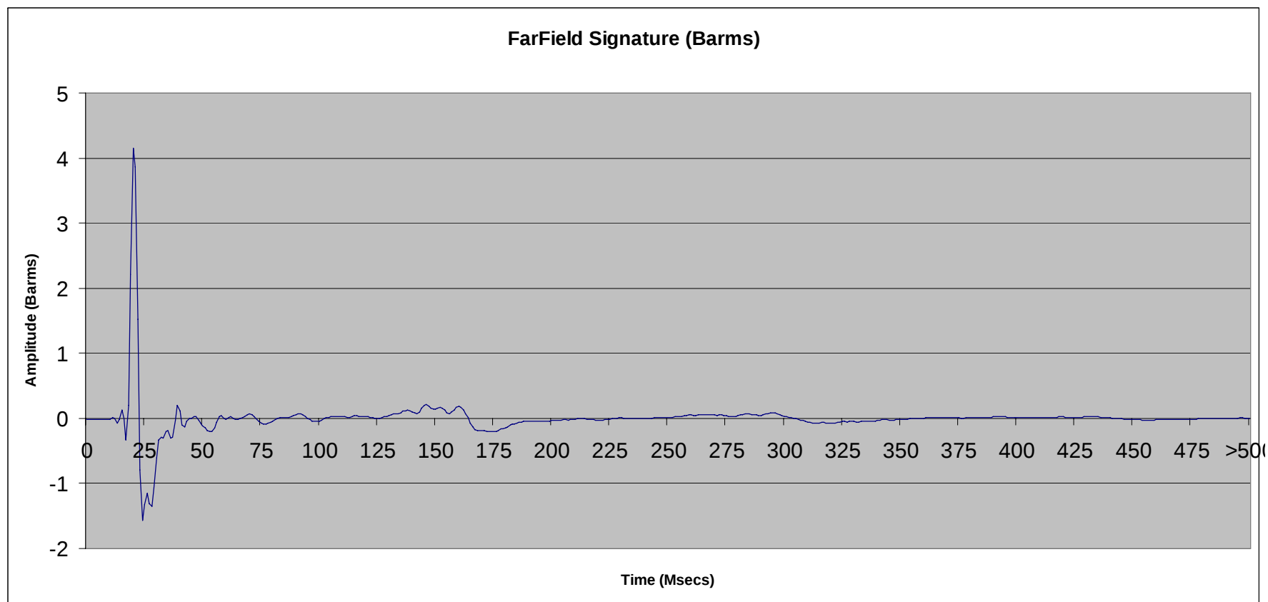
File 2.47: 300 cu in SeaScan Tri-Cluster ® array (# 1 & 2 only) @ 10 ft
