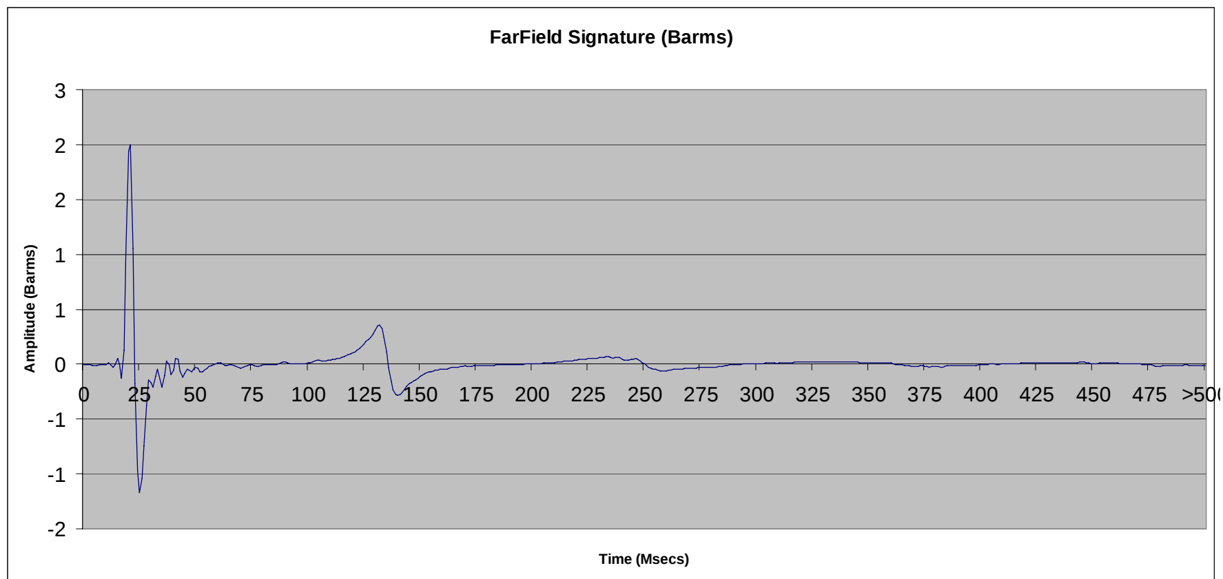
File 2.62: 150 cu in SeaScan Tri-Cluster ® array (# 3 only) @ 10 ft
