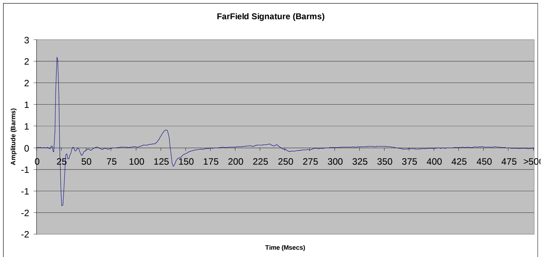
File 2.56: 150 cu in SeaScan Tri-Cluster ® array (# 8 only) @ 10 ft
