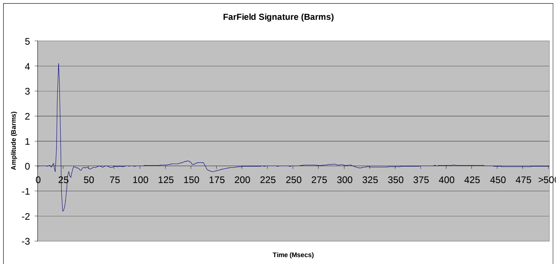
File 2.52: 300 cu in SeaScan Tri-Cluster ® array (# 7 & 8 only) @ 10 ft
