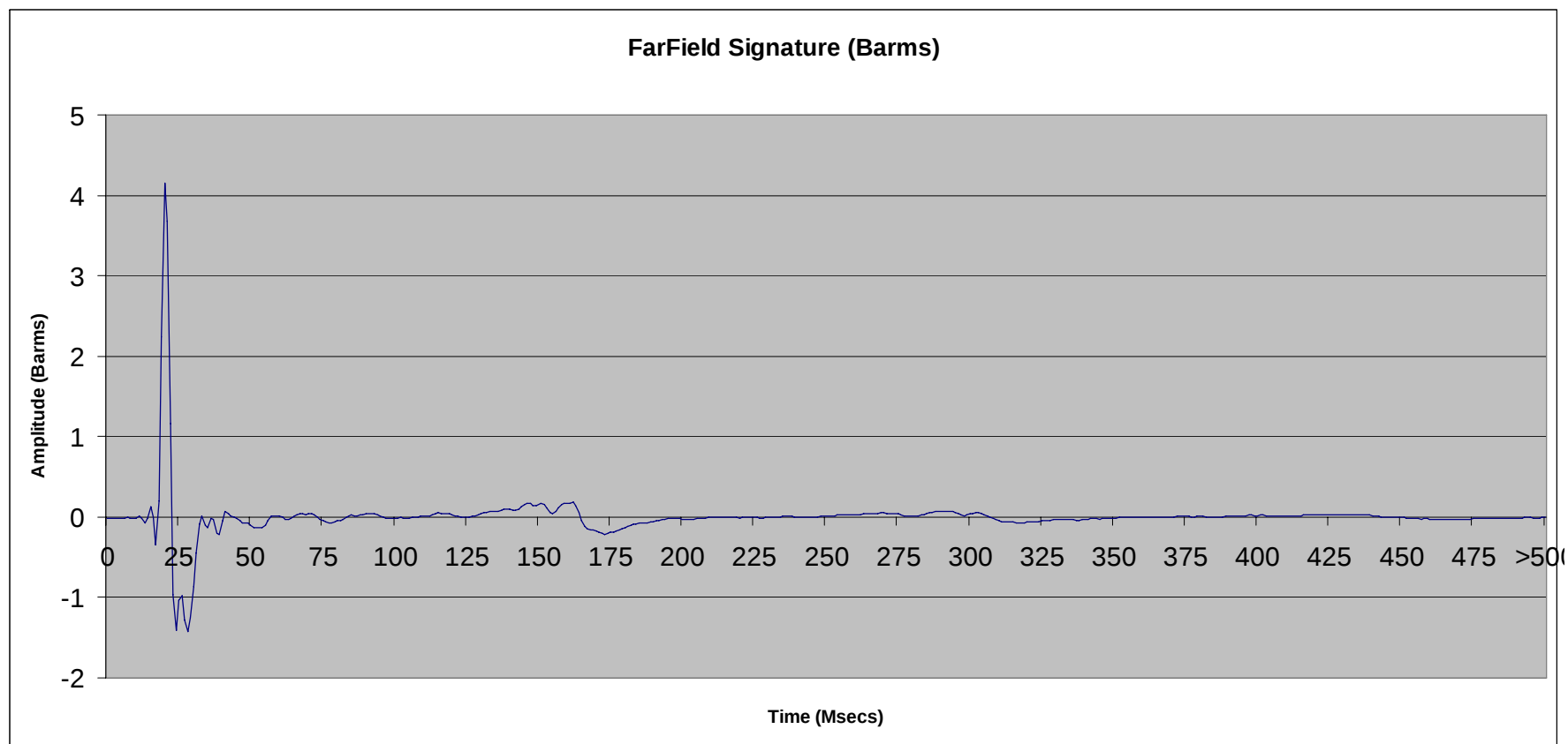
File 2.45: 300 cu in SeaScan Tri-Cluster ® array (# 1 & 2 only) @ 10 ft
