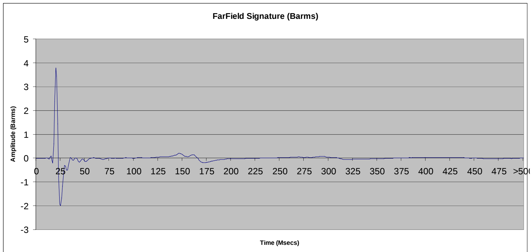
File 2.51: 300 cu in SeaScan Tri-Cluster ® array (# 7 & 8 only) @ 10 ft
