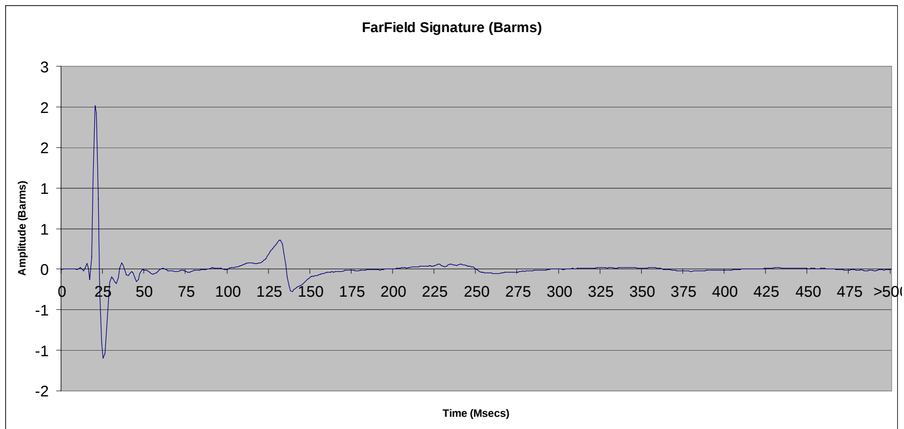
File 2.64: 150 cu in SeaScan Tri-Cluster ® array (# 3 only) @ 10 ft
