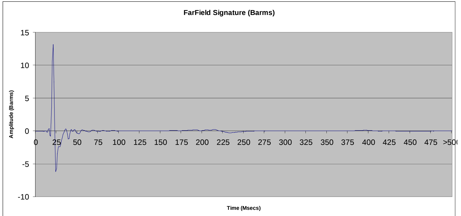
File 2.91: 1200 cu in Single Tri-Cluster ® Tri-Cluster array @ 10 ft
