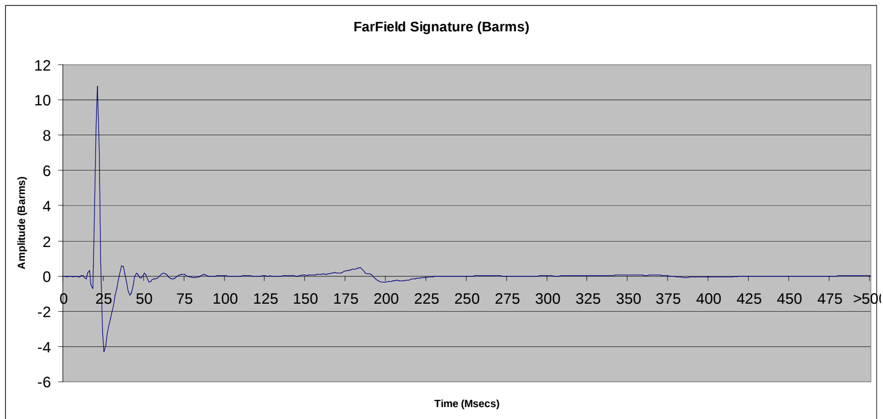
File 2.95: 900 cu in SeaScan Tri-Cluster ® array (#1,2,5,6,7,8 only) @ 10 ft
