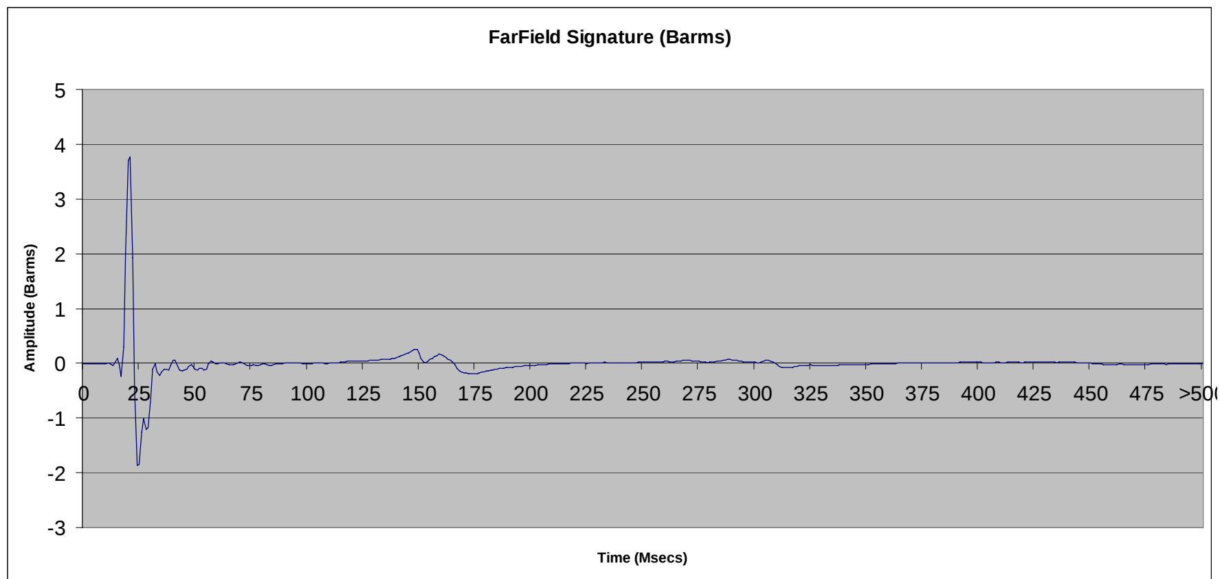
File 2.48: 300 cu in SeaScan Tri-Cluster ® array (# 7 & 8 only) @ 10 ft
