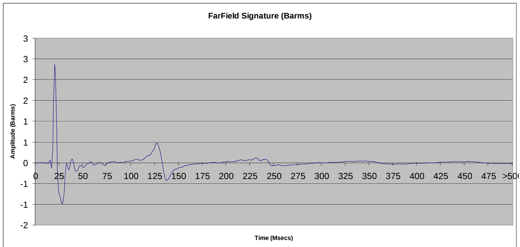
File 2.73: 150 cu in SeaScan Tri-Cluster ® array (#5 only) @ 10 ft
