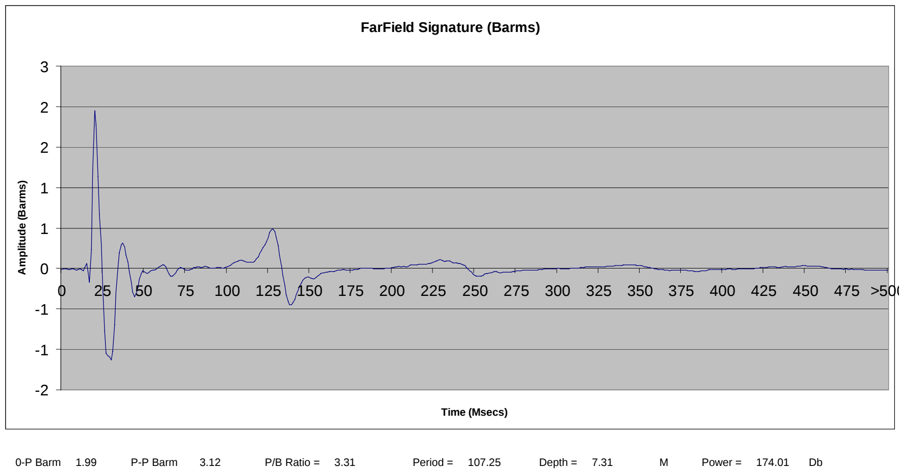
File 2.71: 150 cu in SeaScan Tri-Cluster ® array (#5 only) @ 10 ft
