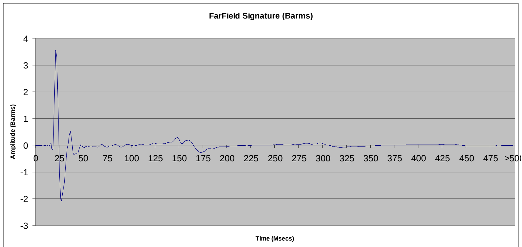
File 2.74: 300 cu in SeaScan Tri-Cluster ® array (#5 & 6) @ 10 ft
