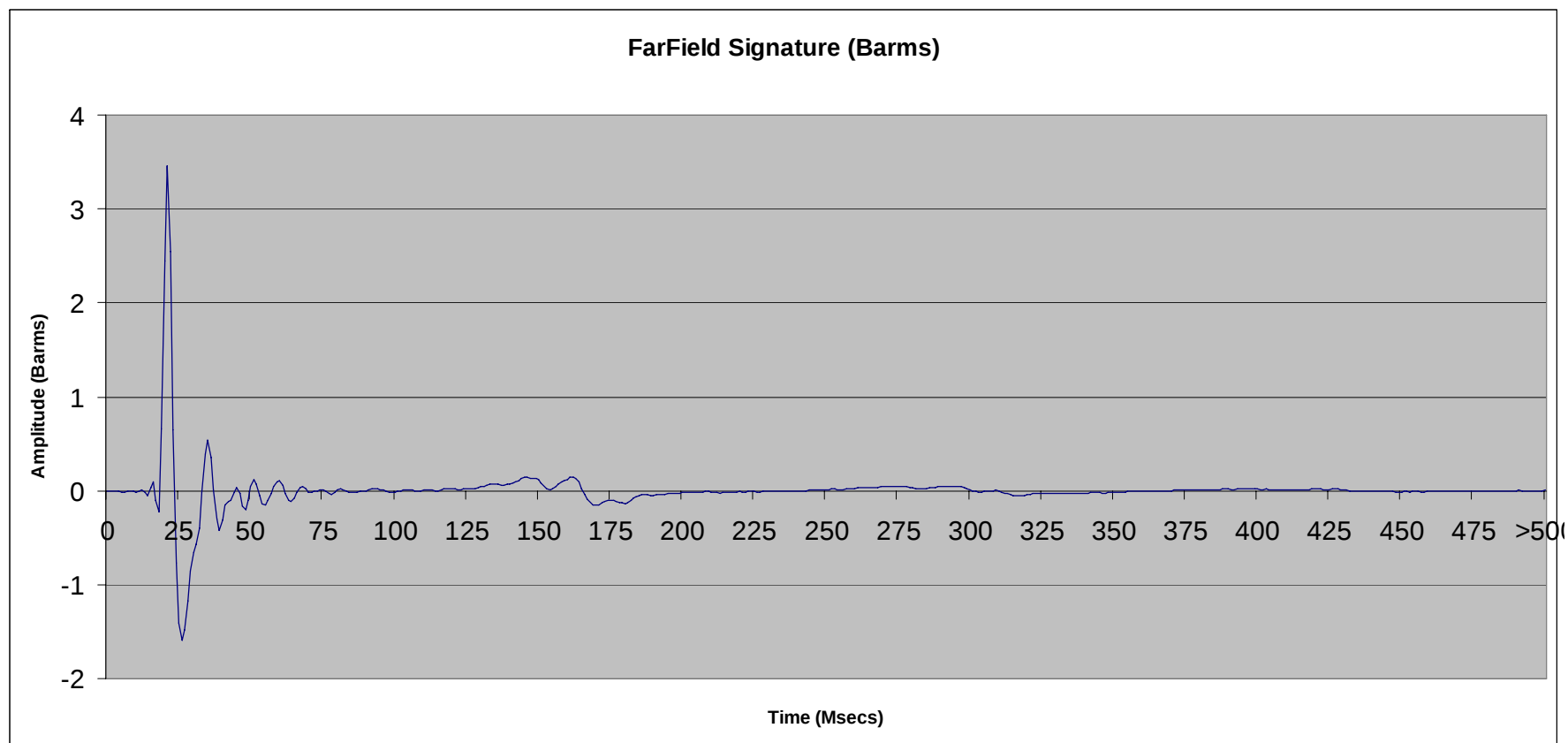
File 2.67: 300 cu in SeaScan Tri-Cluster ® array (# 3 & 4 only) @ 10 ft
