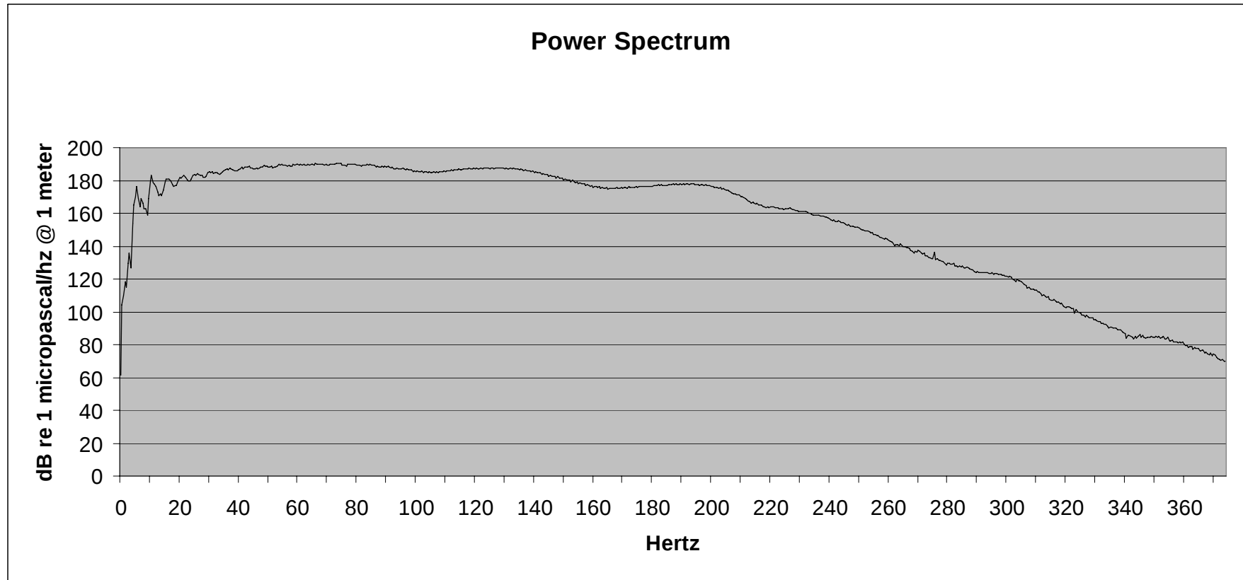
File 2.88: 1200 cu in Single Tri-Cluster ® Tri-Cluster array @ 10 ft
