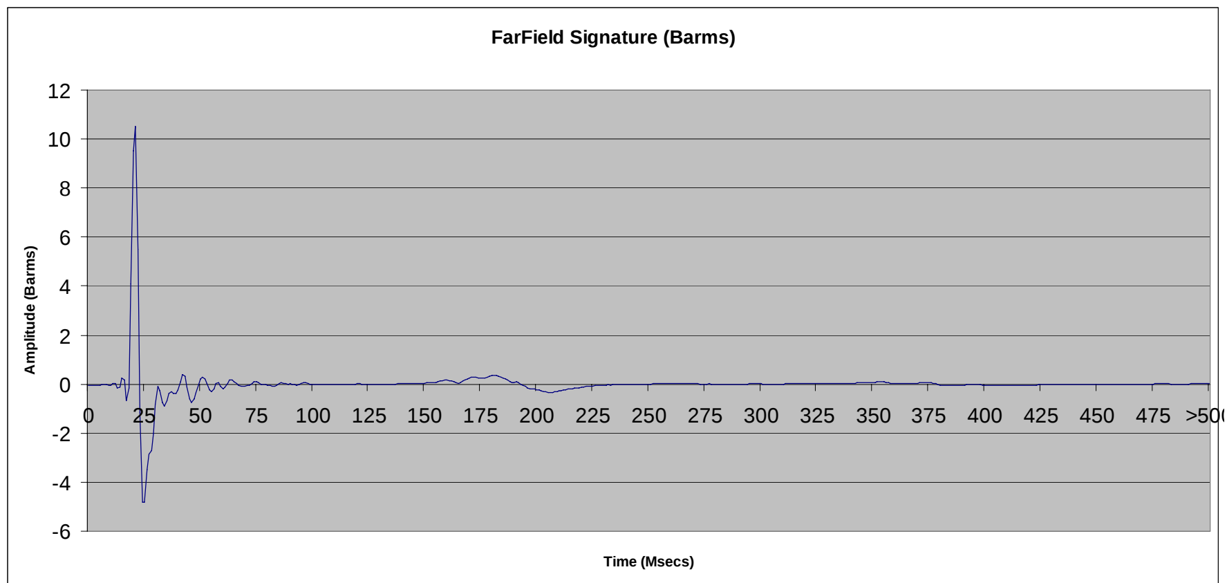
File 2.93: 900 cu in SeaScan Tri-Cluster ® array (#1,2,5,6,7,8 only) @ 10 ft
