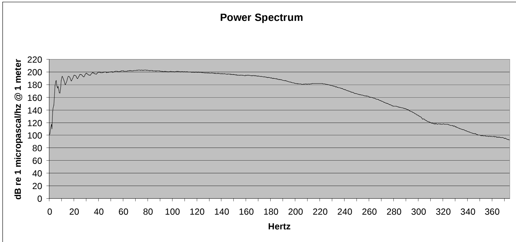
Figure 2: Power Spectrum of the Signature from the 2400 cu in Tri-Cluster ® array (from fig 2.33)
