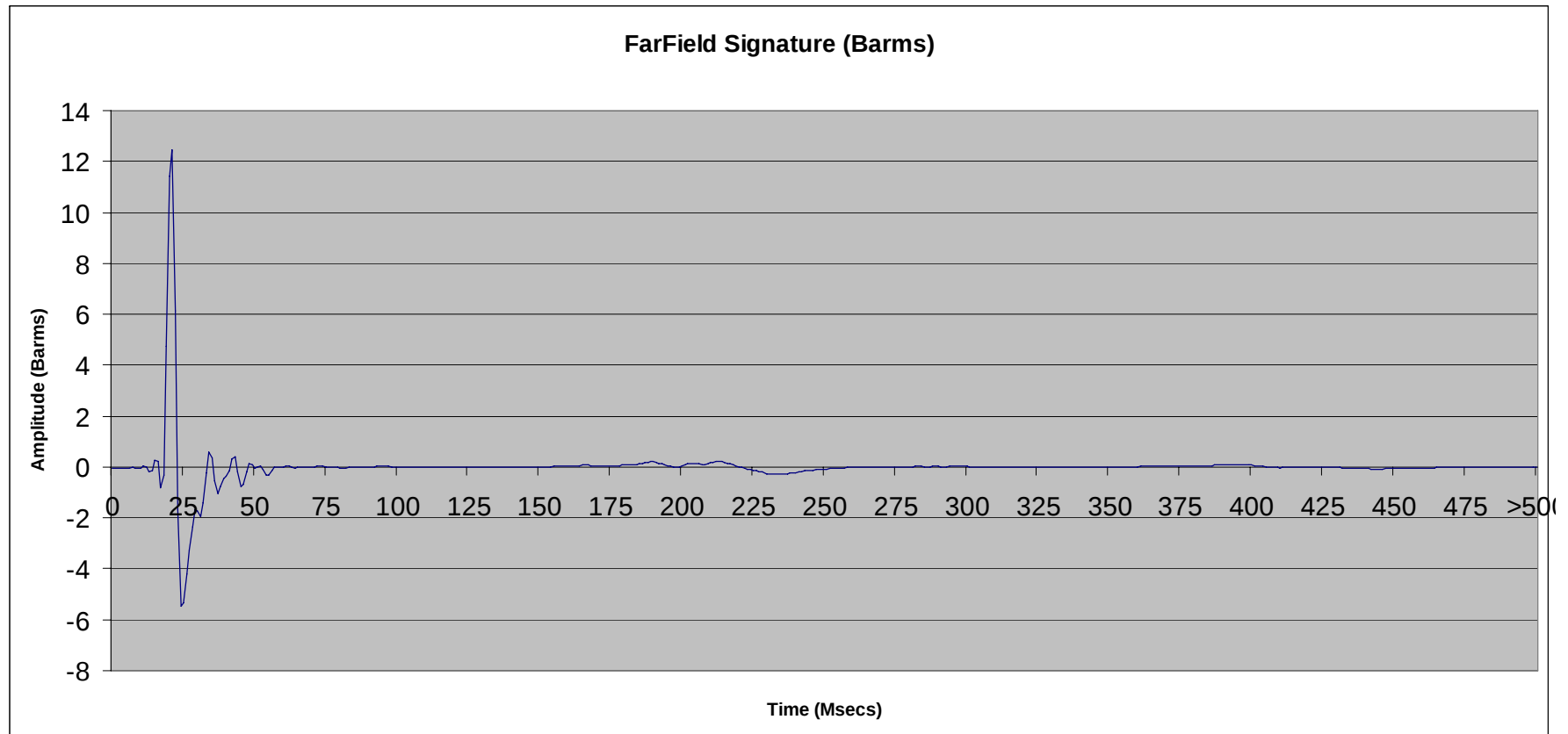
File 2.89: 1200 cu in Single Tri-Cluster ® Tri-Cluster array @ 10 ft
