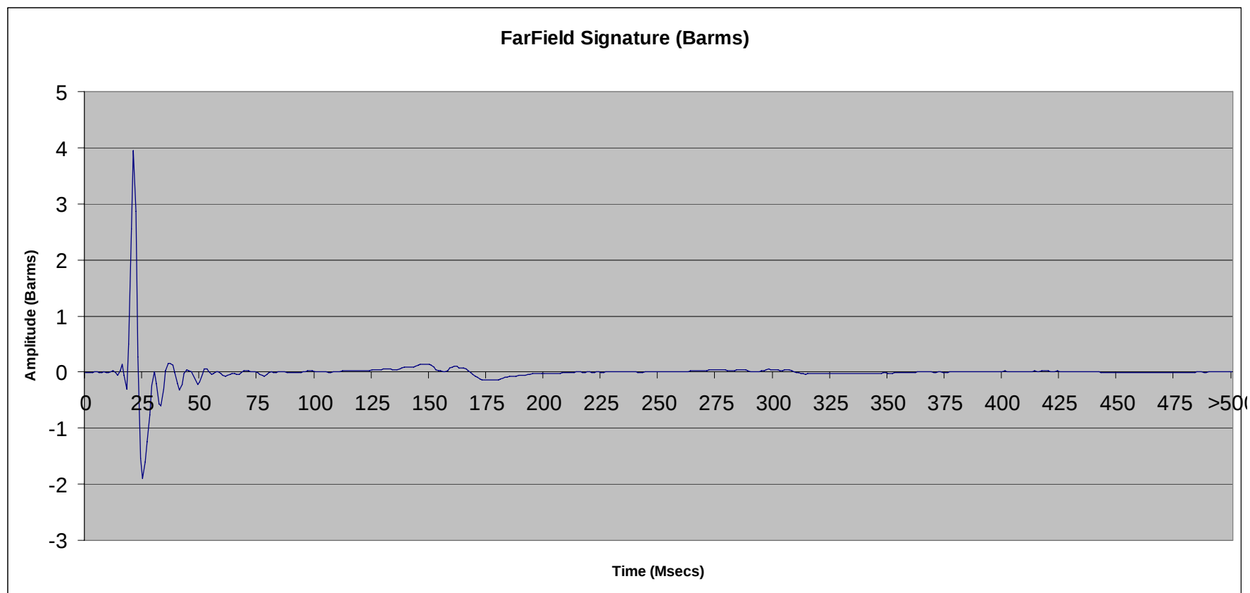
File 2.65: 300 cu in SeaScan Tri-Cluster ® array (# 3 & 4 only) @ 10 ft
