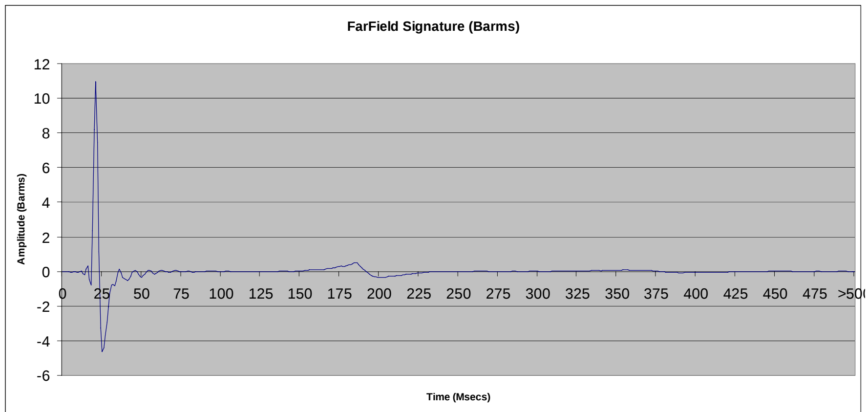
File 2.94: 900 cu in SeaScan Tri-Cluster ® array (#1,2,5,6,7,8 only) @ 10 ft
