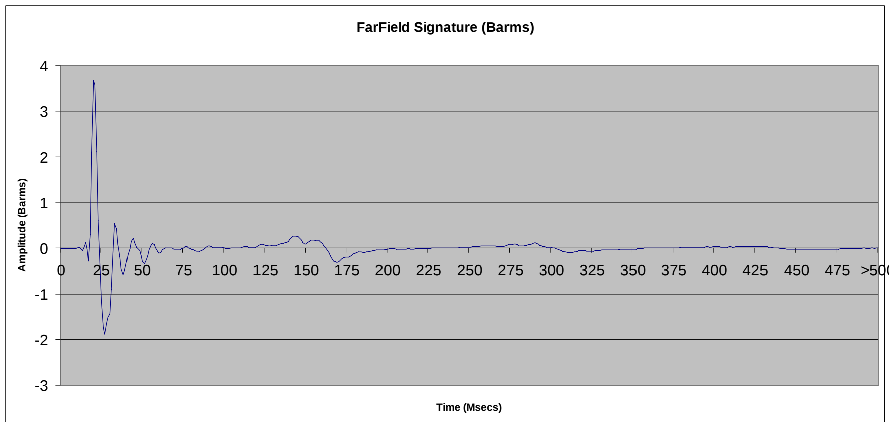
File 2.76: 300 cu in SeaScan Tri-Cluster ® array (#5 & 6) @ 10 ft
