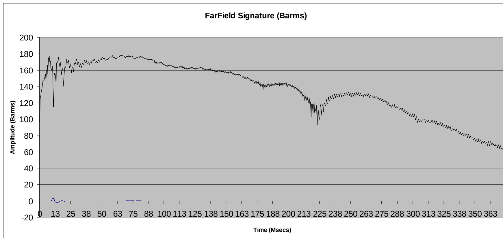
File 2.74: 300 cu in SeaScan Tri-Cluster ® array (#5 & 6) @ 10 ft
