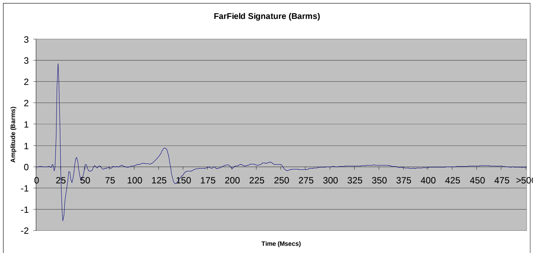
File 2.70: 150 cu in SeaScan Tri-Cluster ® array (#5 only) @ 10 ft
